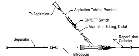
Figure 1 – Assembled Aspiration System with Penumbra Separator
